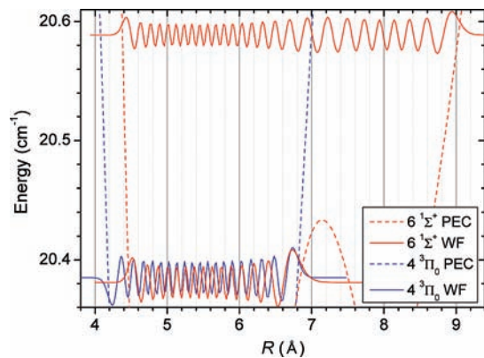
Figure 7. Vibrational wave functions of the v_{\Pi} = 37 level at 20385 cm -1 (blue solid line) and the two v_{\Sigma} levels at 20381 and 20589 cm -1 (red solid lines), and PECs of the 4^3\Pi_0 (blue dotted line) and 6^1\Sigma^+ (red dotted line) states.
