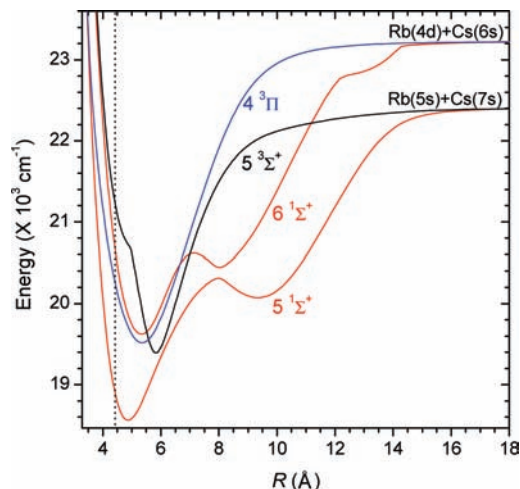
Figure 1. Nonrelativistic ab initio PECs of RbCs for the 5^1\Sigma^+ , 6^1\Sigma^+ , 5^3\Sigma^+ , and 4^3\Pi states from ref 18. The vertical dotted line represents the FC region ( R_e of the X^1\Sigma^+ state, 4.379 Å from ref 18). The origin of the ordinate axis is set to the potential minimum of the X^1\Sigma^+ state.
